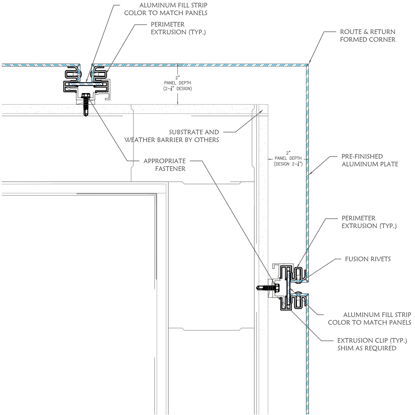
FORMED ACM OUTSIDE CORNER DETAIL
